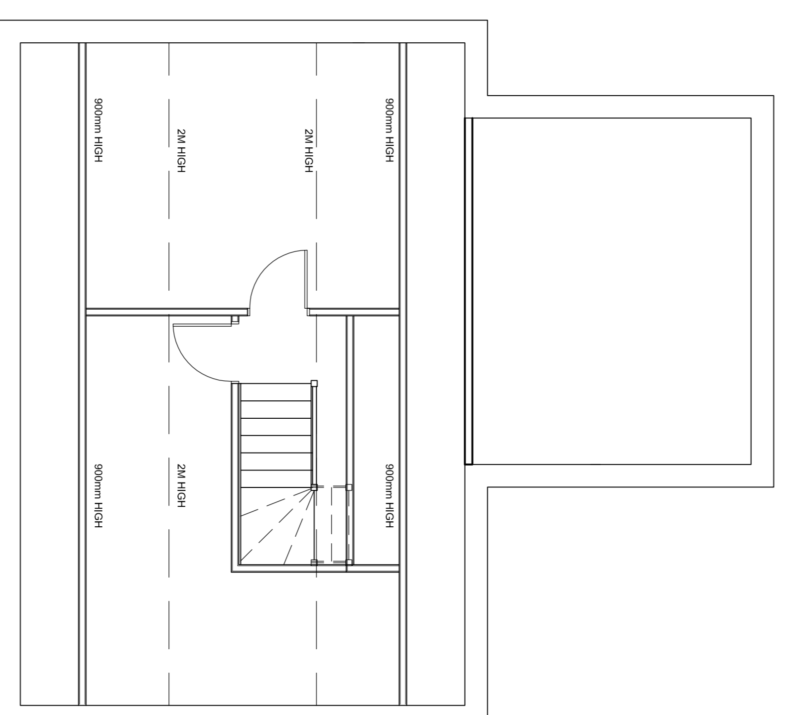
SECOND FLOOR PLAN (INDICATIVE)
